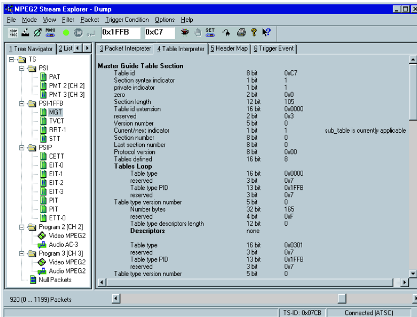
Fig. 2: Clear representation of transport stream structure with Tree Navigator and Table Interpreter (ATSC)
